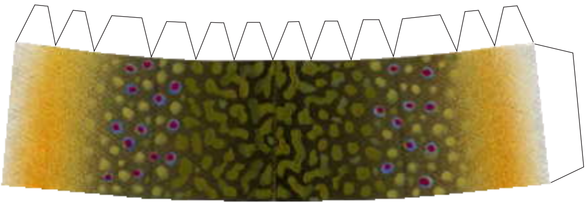
Brook trout ( Salvelinus fontinalis ) 1
